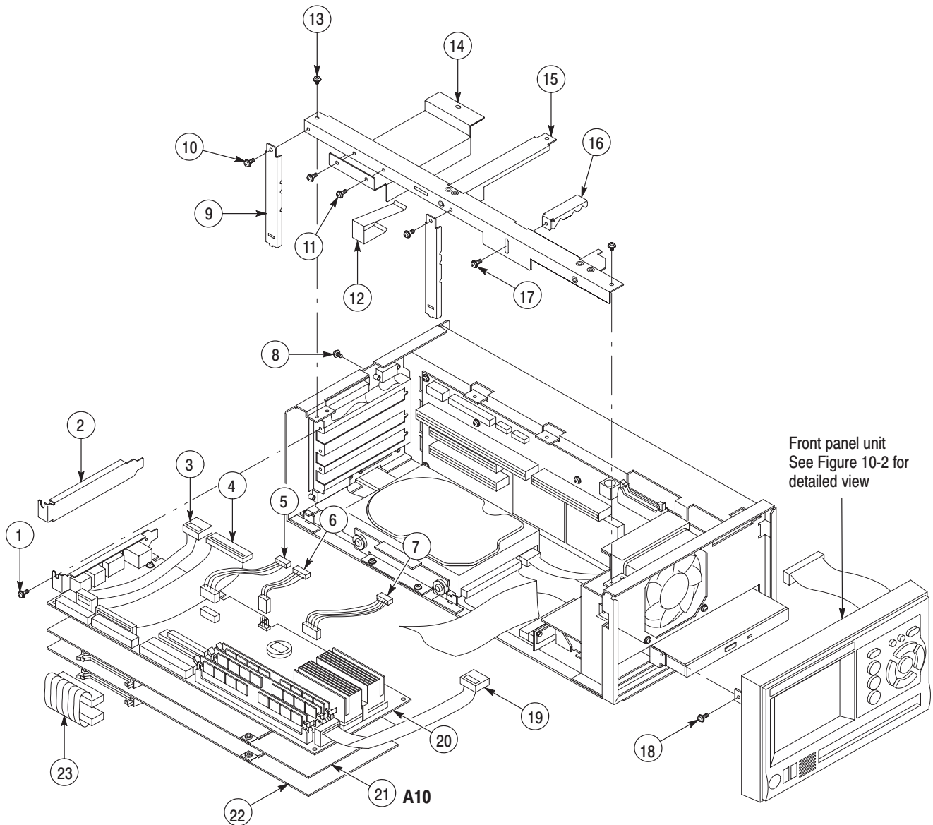
Figure 10-5: Internal modules (3)
