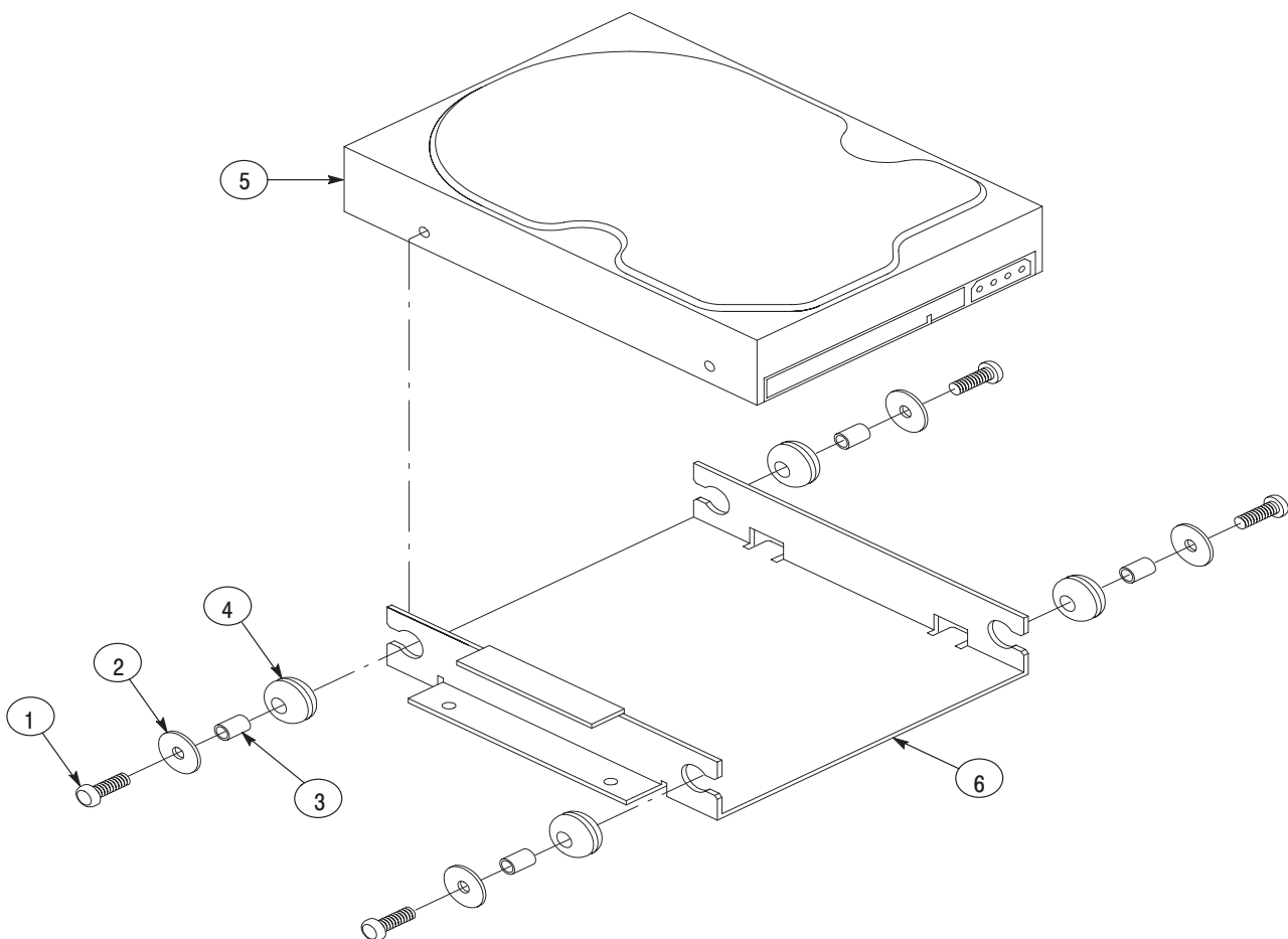
Figure 10-7: Hard Disk Drive unit
