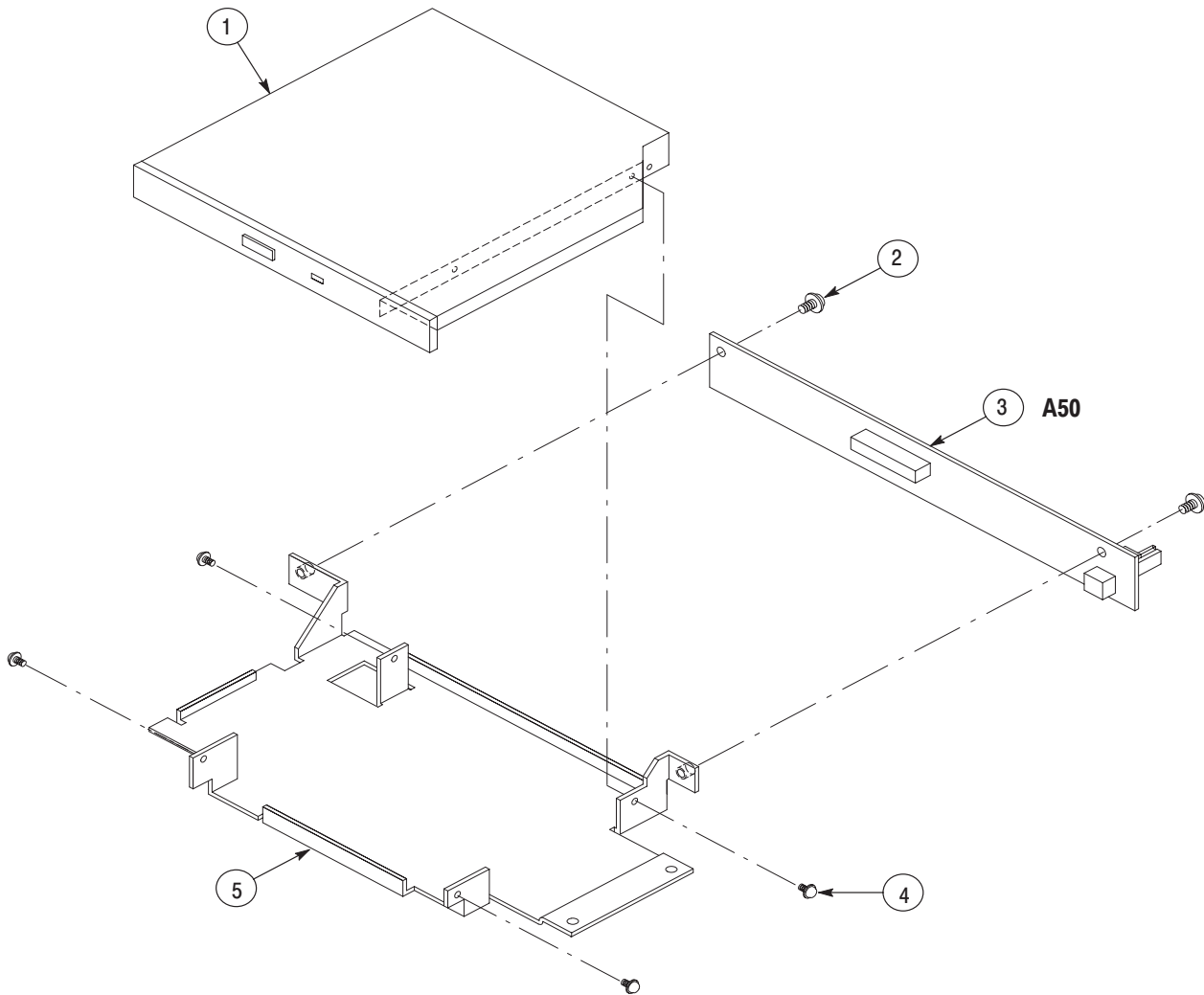
Figure 10-6: CD-ROM unit
