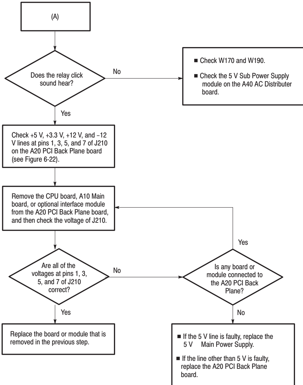
Figure 6-19: Troubleshooting procedure (3)
