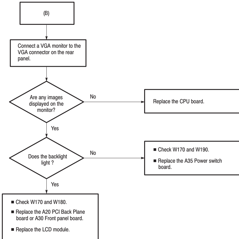
Figure 6-20: Troubleshooting procedure (4)
